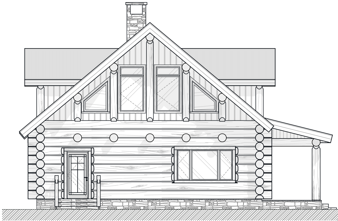
Front Elevation, Left Elevation
